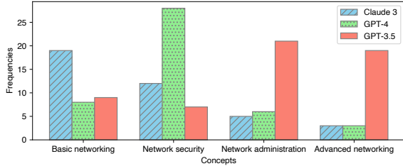
Figure 5: Frequency of misconceptions across different networking topics.
